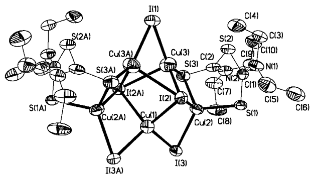
Fig. 1 Structure of [\text{Cu}_5\text{L}^{\text{Et}_2\text{I}_5}] \cdot \text{EtOH} \cdot \text{MeCN} 1 and numbering scheme with 50% displacement ellipsoids for non-hydrogen atoms
